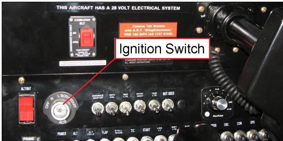
Figure 1-29 Ignition Switch
