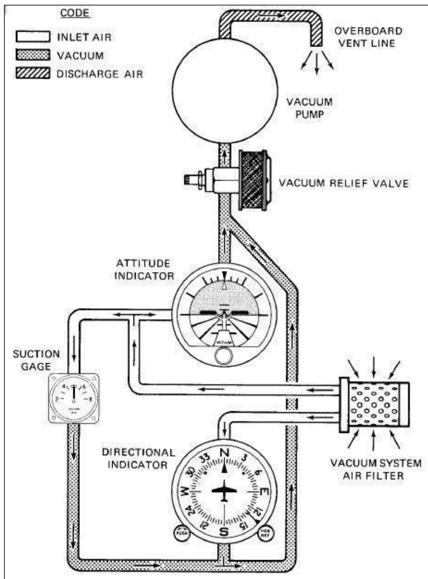
Figure 1-55 Vacuum System
