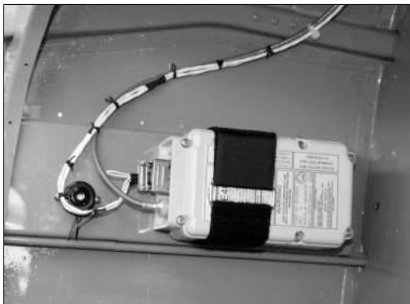
Figure 1-63 Artex ME406
