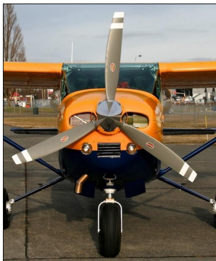
Figure 1-24 Hartzell Propeller
