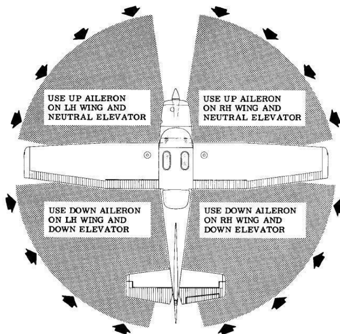
Figure 2-11 Control Positions during Taxi
