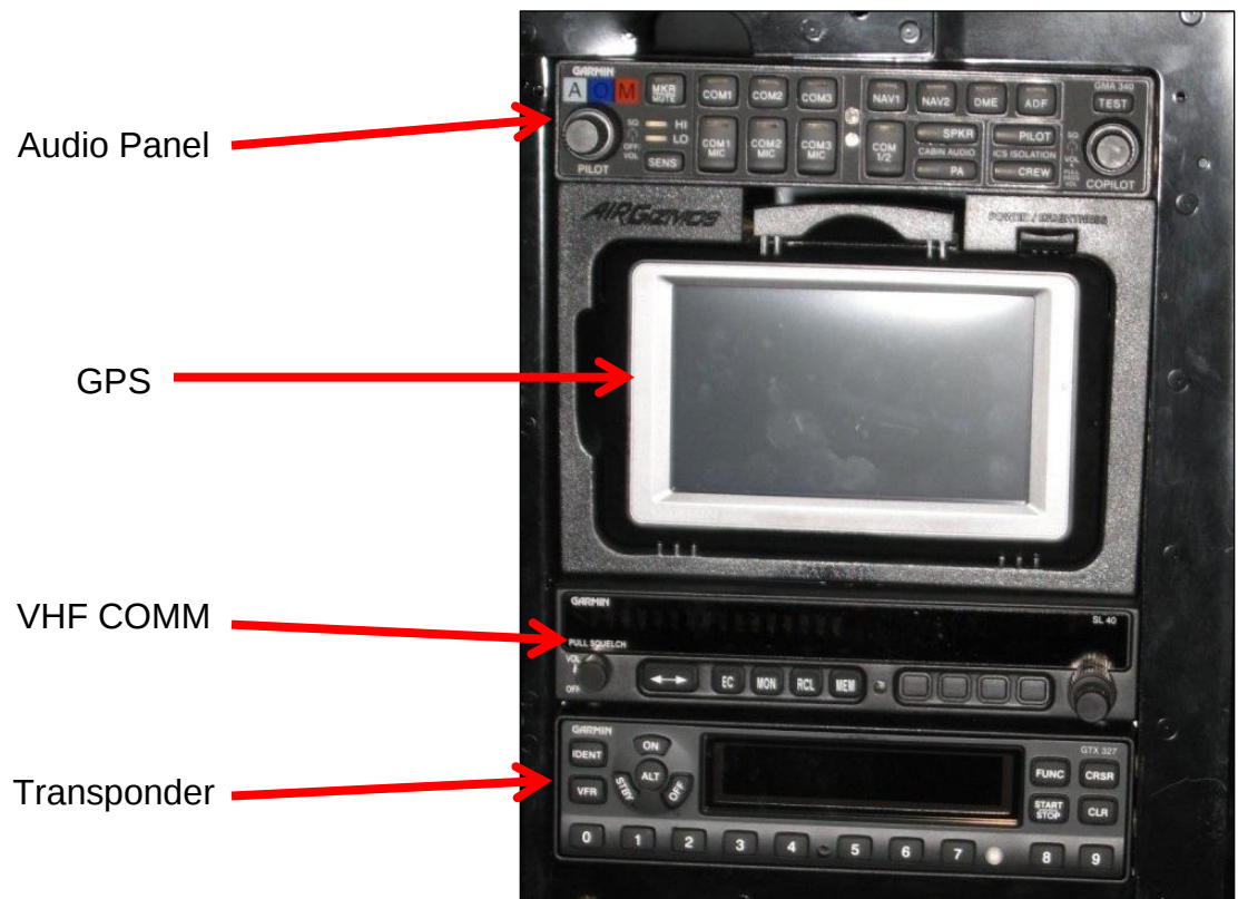
Figure 1-58 Avionics Suite
