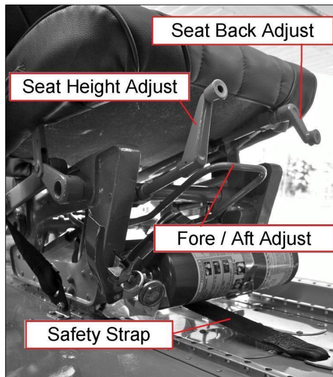
Figure 1-12 Seat Controls
