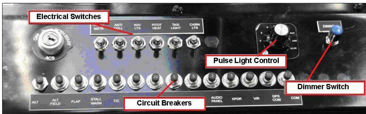
Figure 1-50 Electrical Panel
